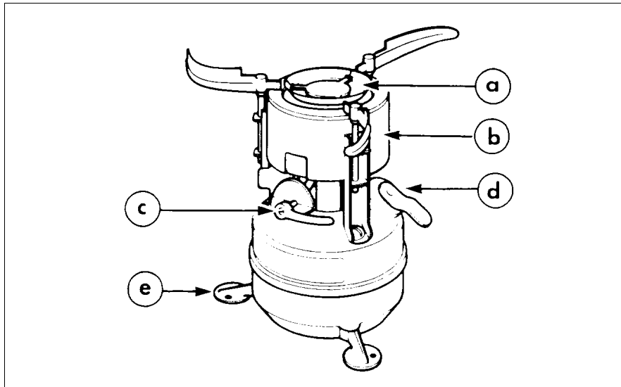
Figure 2-7 Stove M 1950
