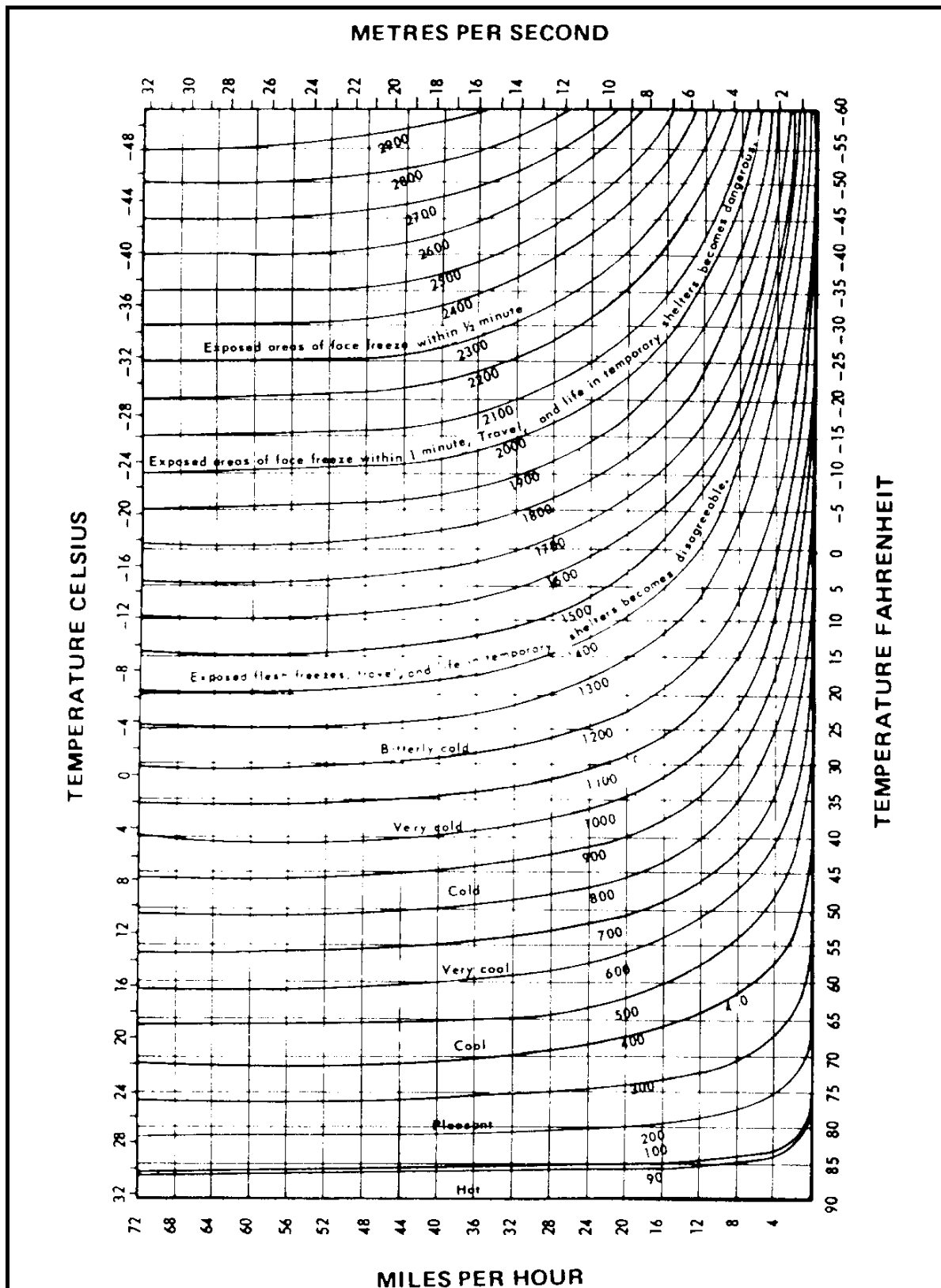
Figure 1-2 Windchill Graph
