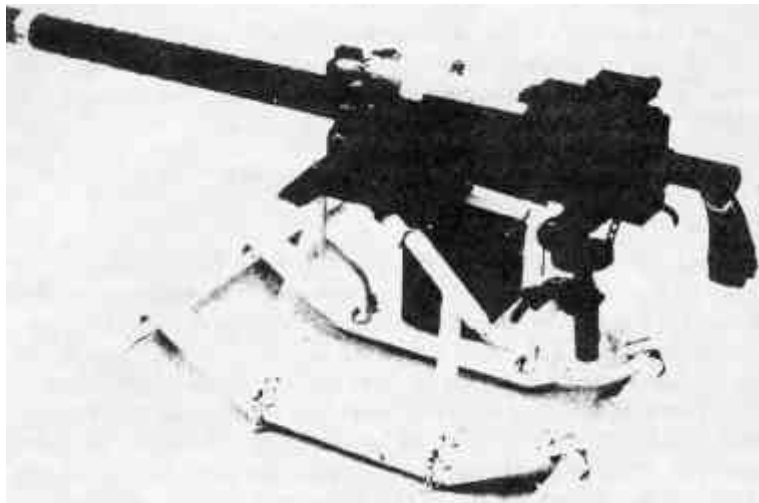
Figure 4-11 Machine-gun Mounted on a Toboggan
