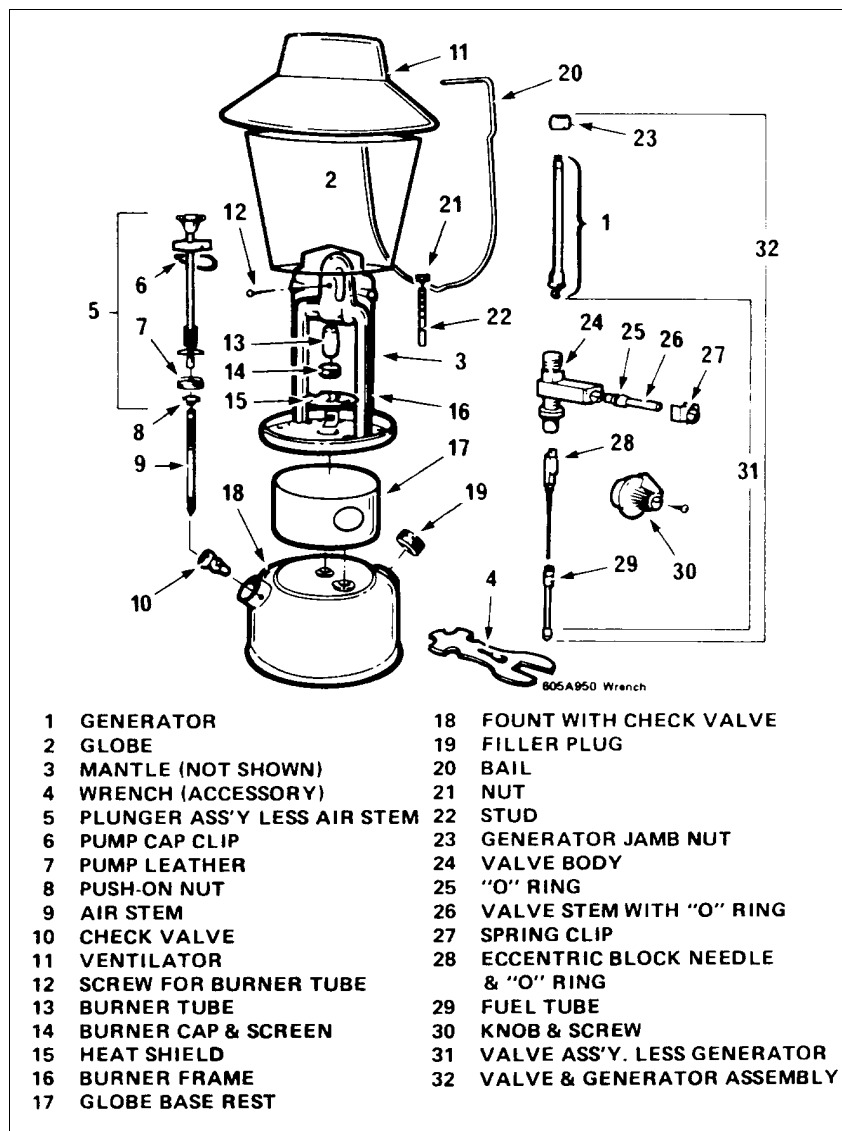
Figure 2-6A Coleman Lantern 621 B
