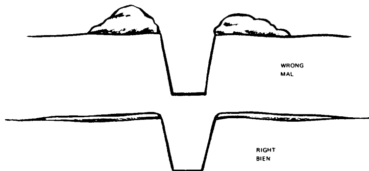
Figure 4-19 Snow Trench
