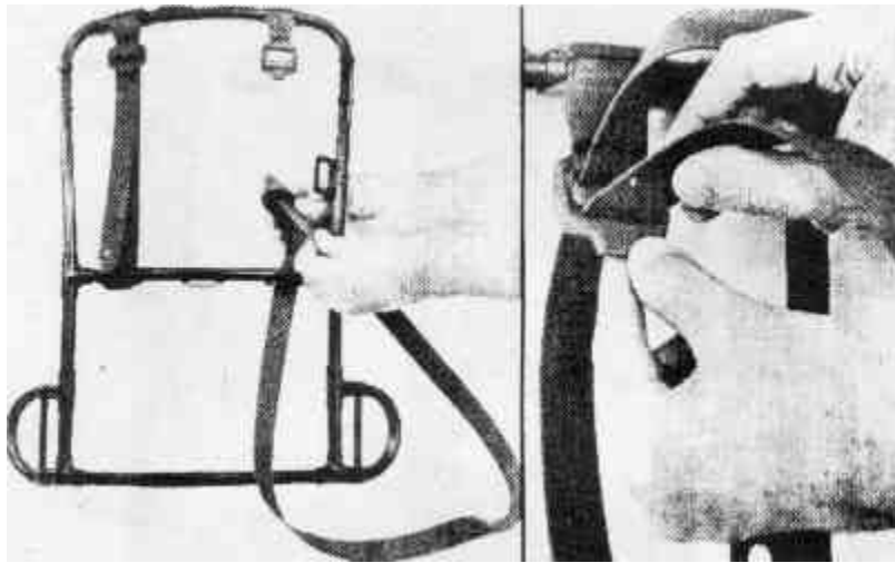
Figure 2-4B Assembly
