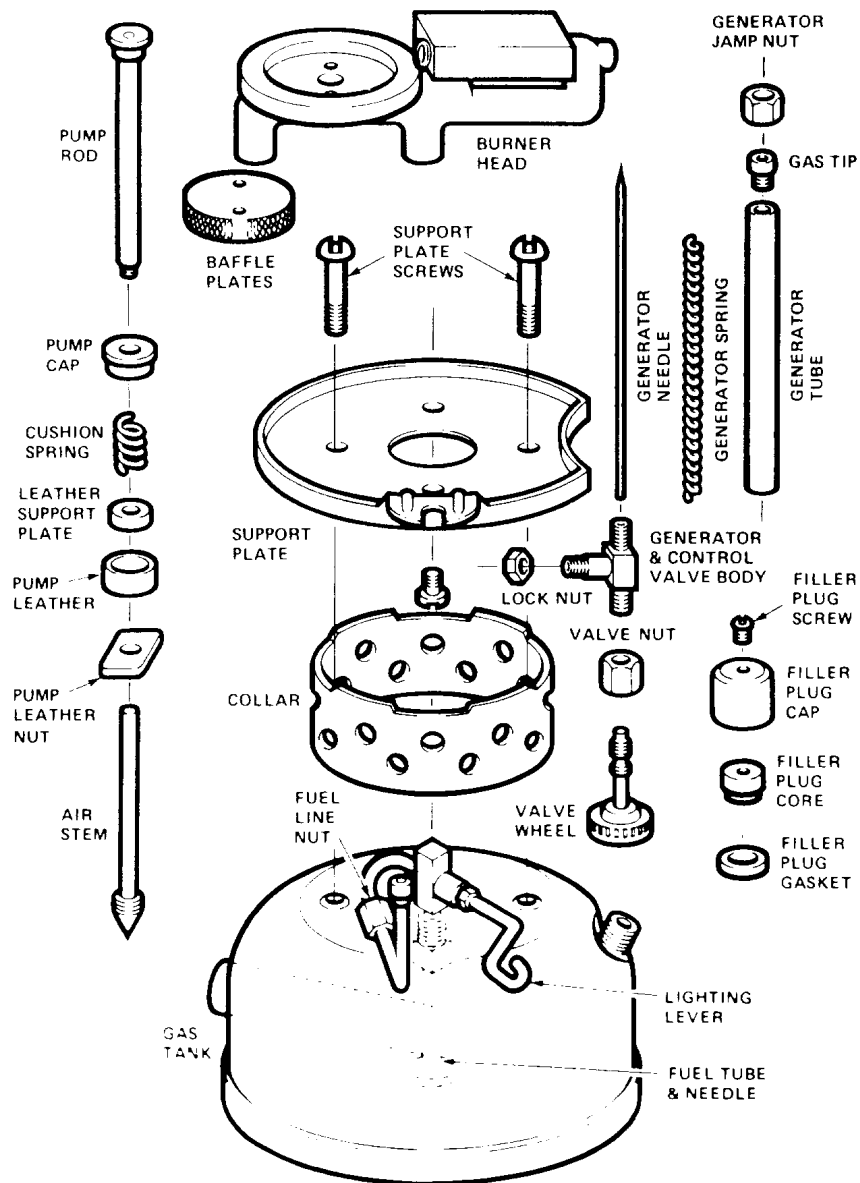
Figure 2-8A Stove C1B1
