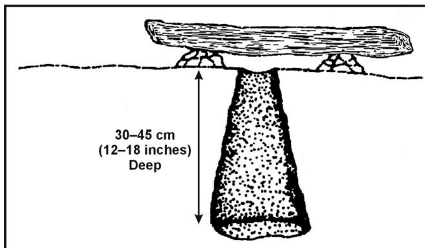
Figure 8-17. Bottle Trap
