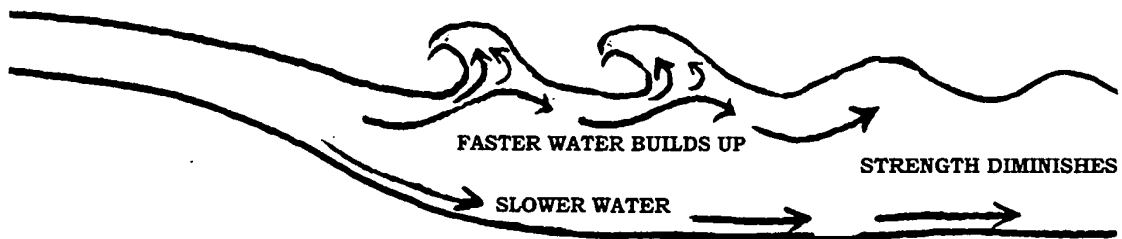
STANDING WAVES/HAYSTACKS
