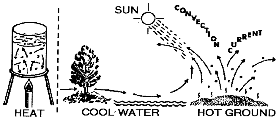
CONVECTION EFFECTS
