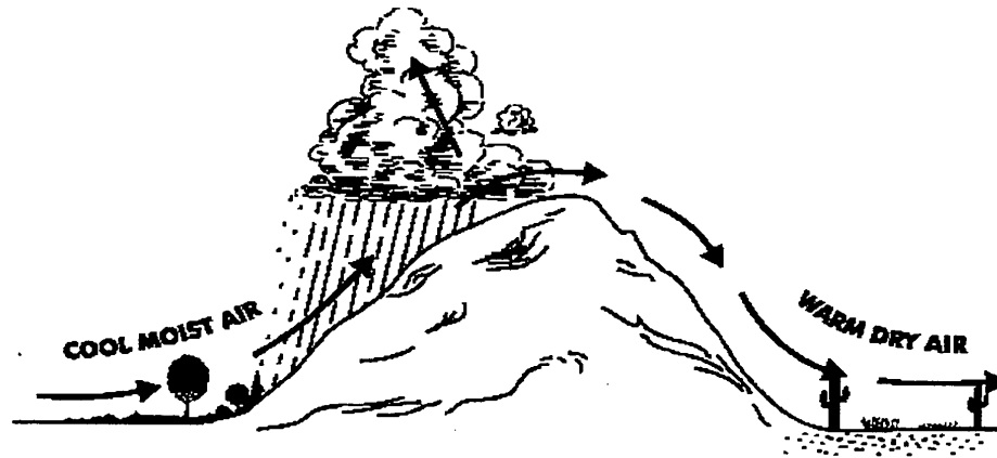
OROGRAPHIC UPLIFT
